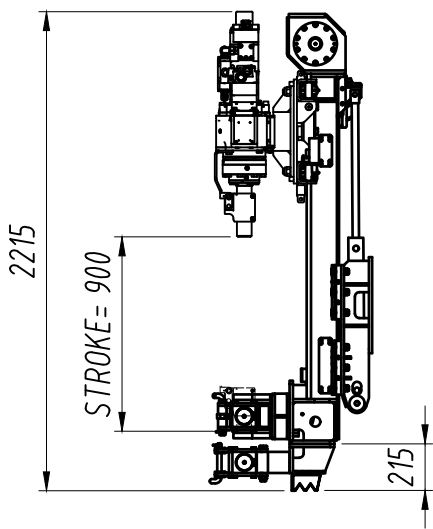
CID 250 MAST - STROKE= 900 ROD BREAKER CLAMP 70÷188 CLAMP 70÷188
