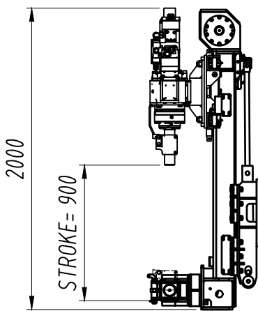
CID 250 MAST - STROKE= 900 ROD BREAKER CLAMP 70÷188
