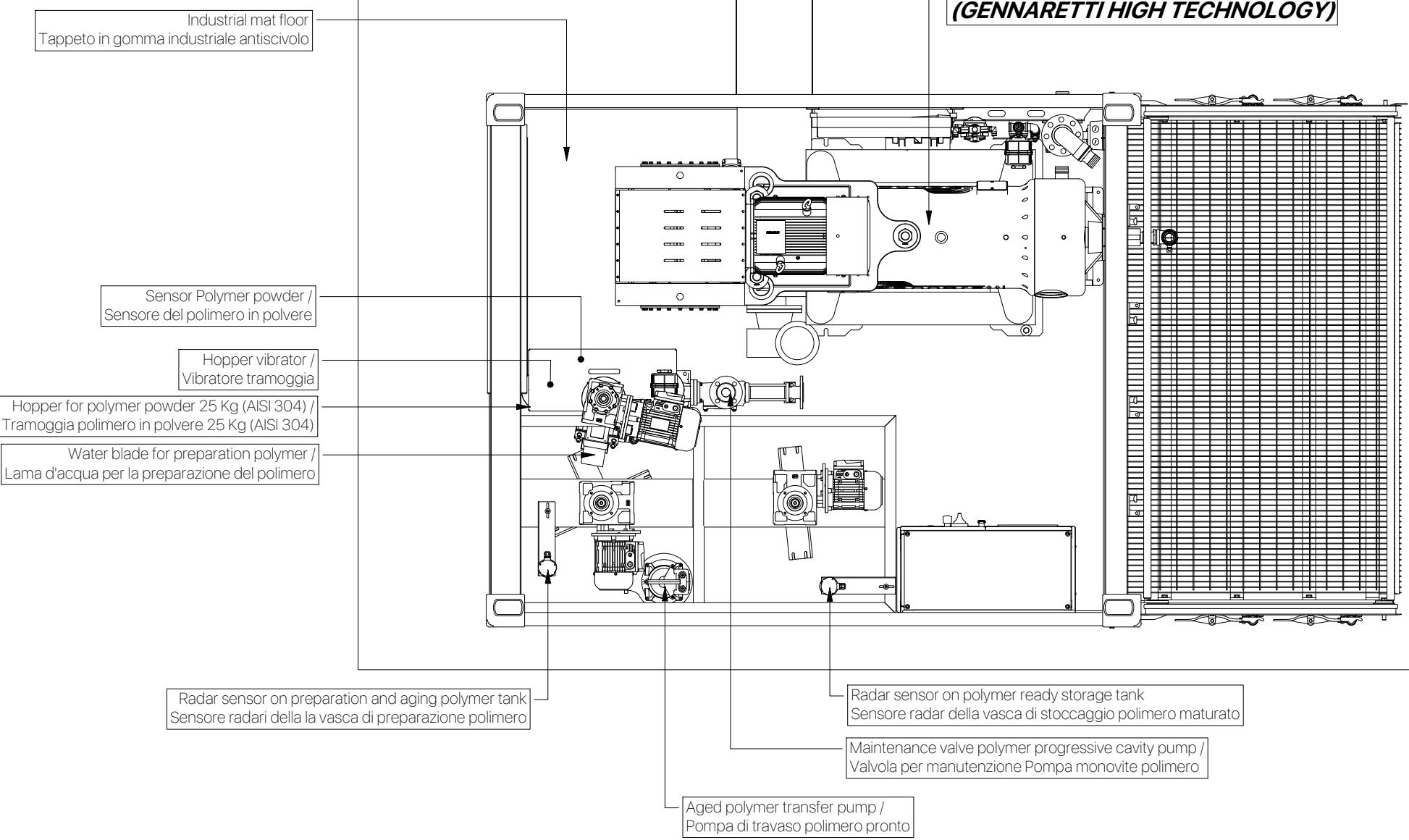
TOP VIEW ( 1 : 25 )
