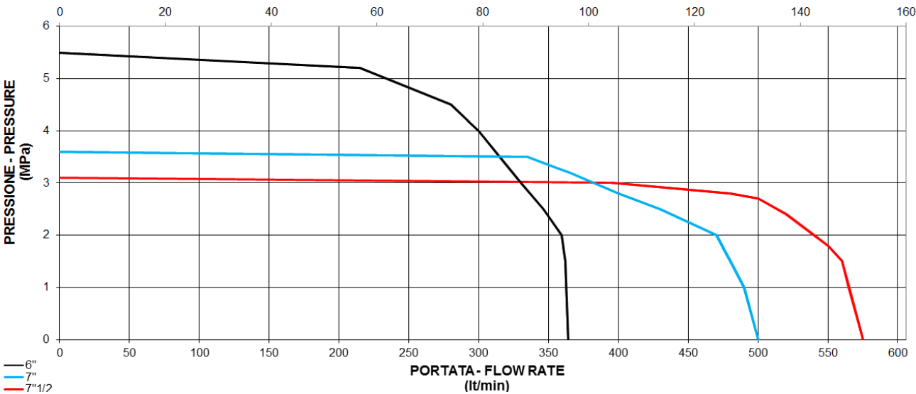
DIAGRAMMA PORTATA - PRESSIONE PRESSURE-FLOW RATE DIAGRAM
